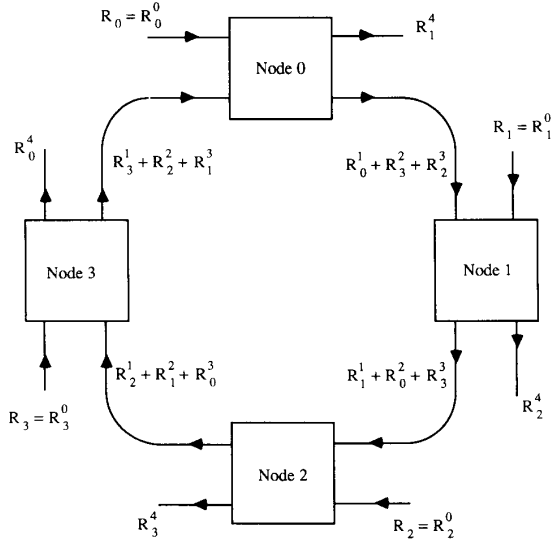
Fig. 2. Network example 2.
