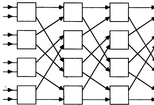
Fig. 4. Omega network.
